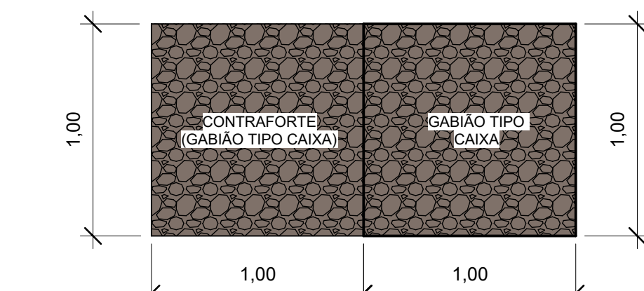
5 1 : 25 CORTE 1 GABIÃO 4/5/6/7
