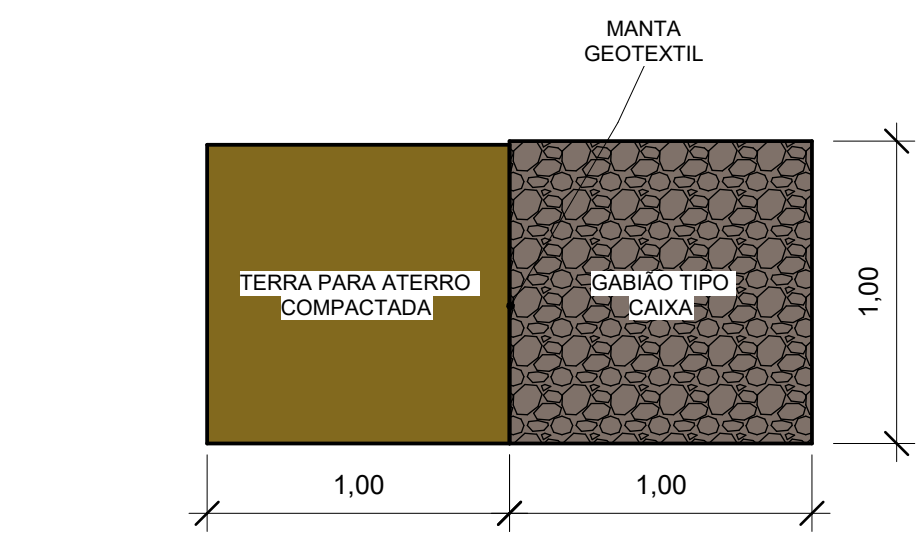
6 1 : 25 CORTE 2 GABIÃO 4/5/6/7
